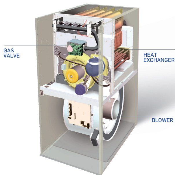
PERFORMANCE™ 96 GAS FURNACE
