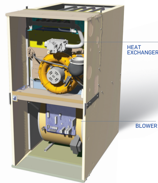
COMFORT™ 96 GAS FURNACE
